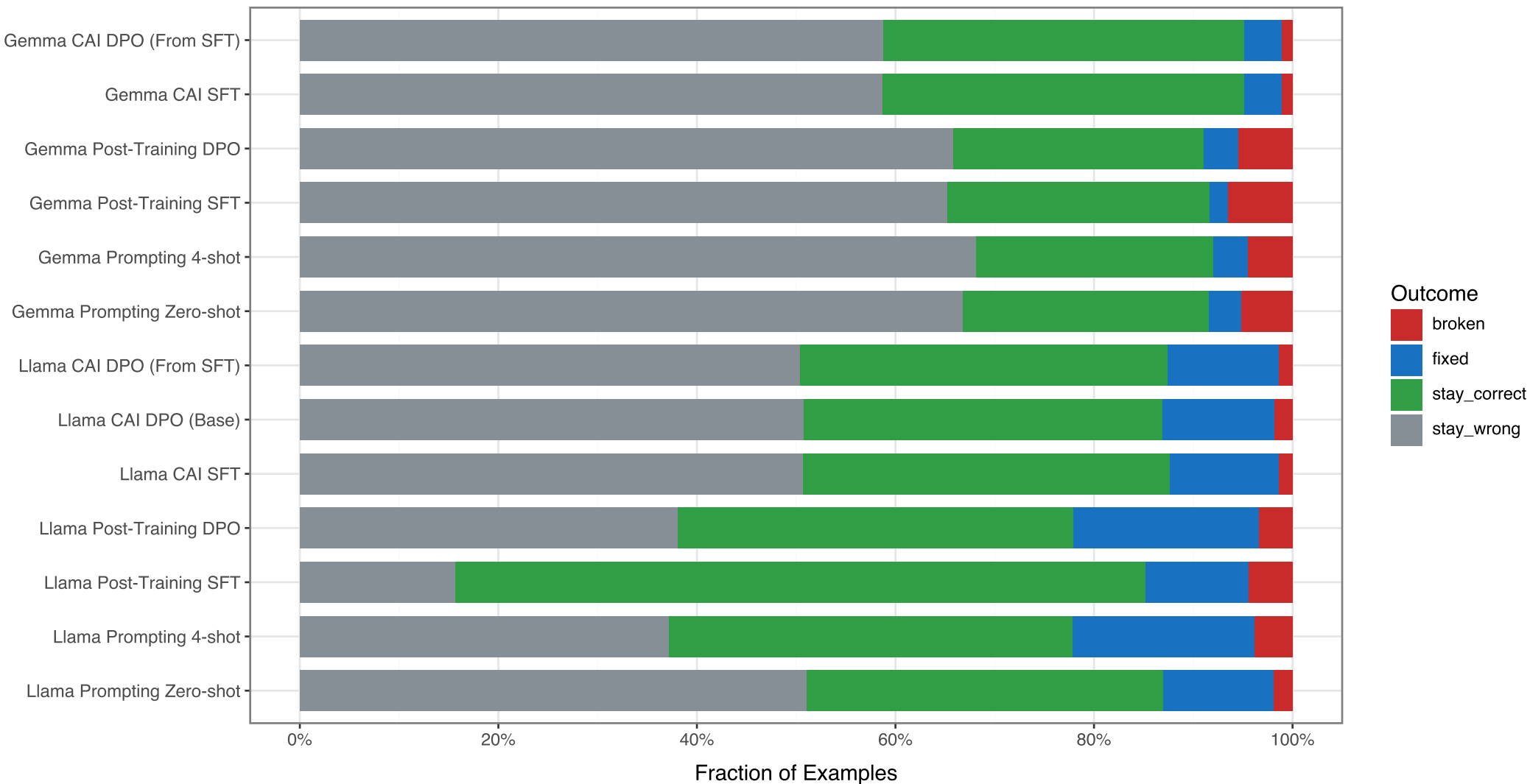
Normalization Outcome Breakdown on When2Call (No Probe)
